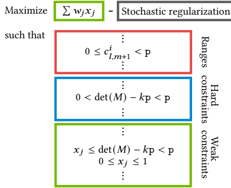
Fig. 4. Anatomy of an Integer Linear Program (ILP): To grow the matrices C_i according to Theorem 5.2, the values of the c_{l,m+1}^i in the last column of their respective C_i are determined by solving an ILP, which consists of an objective function to maximize subject to a set of constraints. The range constraints enforce that c_{l,m+1}^i \in \{0, \dots, p-1\} and the hard uniformity constraints enforce a non-zero determinant to guarantee the design constraints of stratification, net, and sequence properties as introduced in Section 4. Remember that matrices M are constructed from first rows of the C_i matrices and hence include some of the c_{l,m+1}^i . Indicated by x_j = 1 , a satisfied weak constraint adds its weight w_j to the objective function. Otherwise, a zero determinant comes along with x_j = 0 . The stochastic regularization term is detailed in Equation (9).
